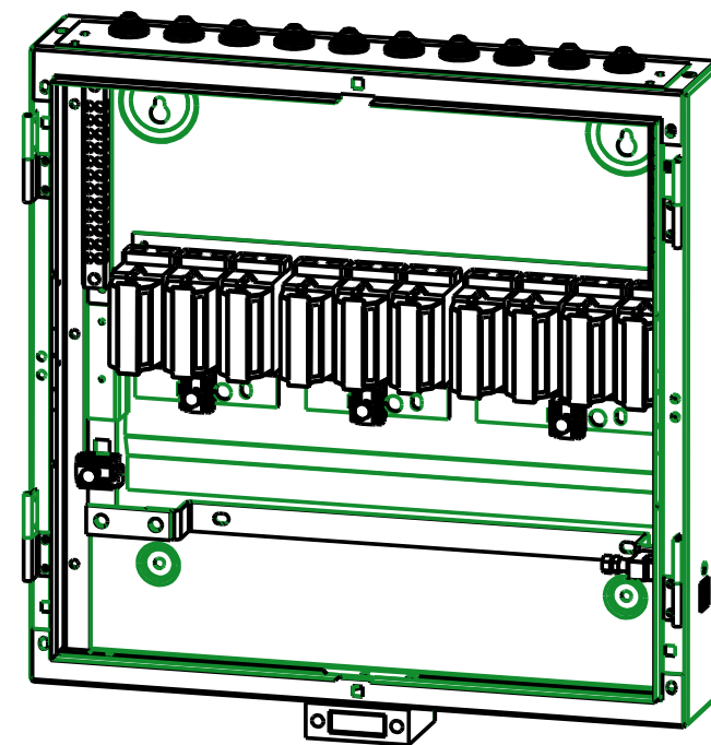
ISOMETRIC VIEW WITH DOOR AND CABLE SCREEN REMOVED
